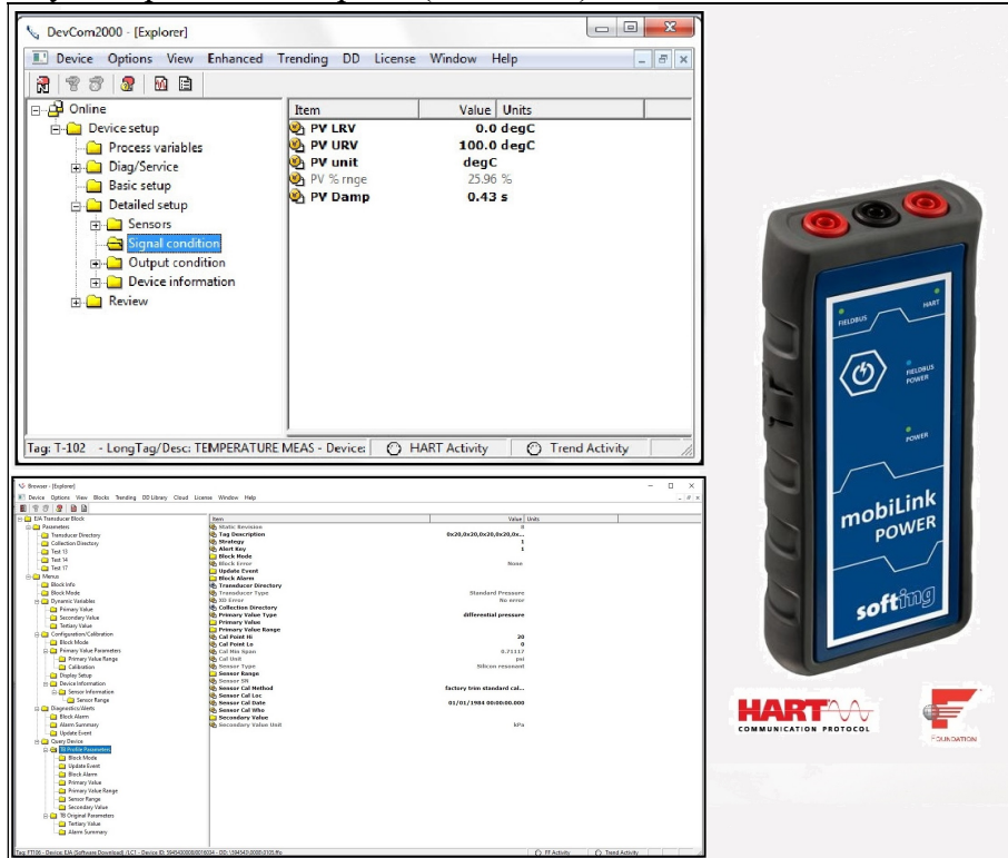
DevCom2000 HART Software + DevComFF.Win FF Software + MOBI-FF-PWR HART and FF Modem with Integrated Power Supply
